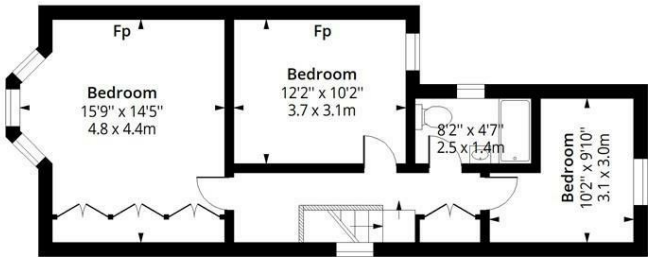
First Floor
